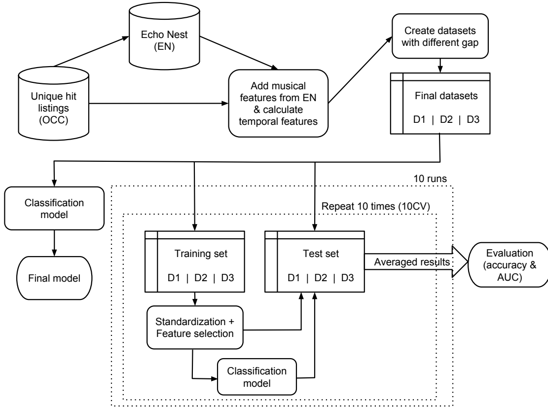
Figure 3: Flow chart of the experimental setup.
