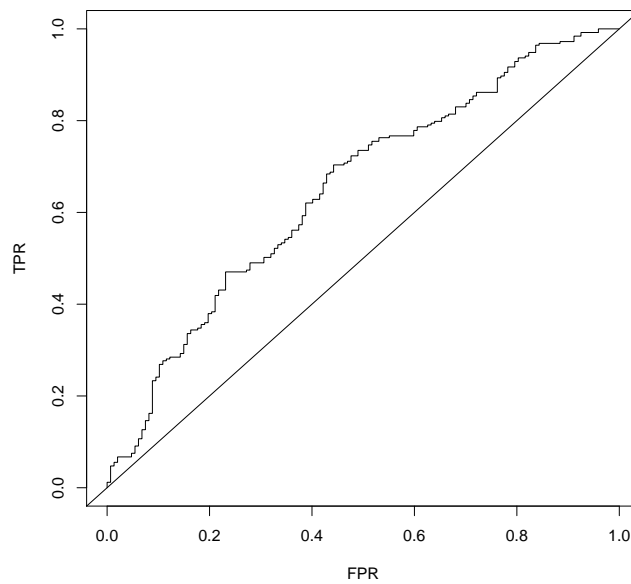
Figure 8: ROC for Logistic regression
