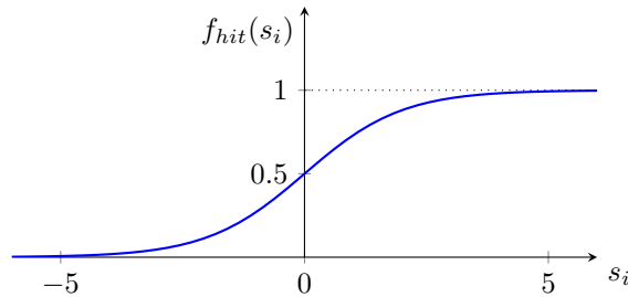
Figure 6: Probability that song i is a dance hit.
