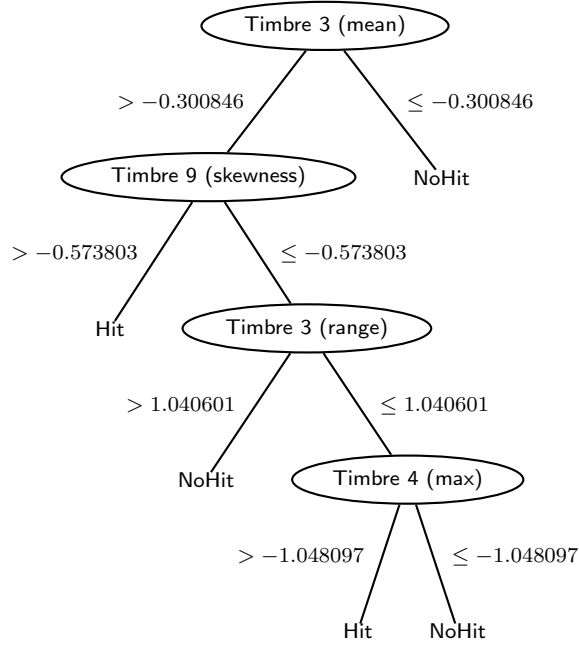
Figure 5: C4.5 decision tree.
