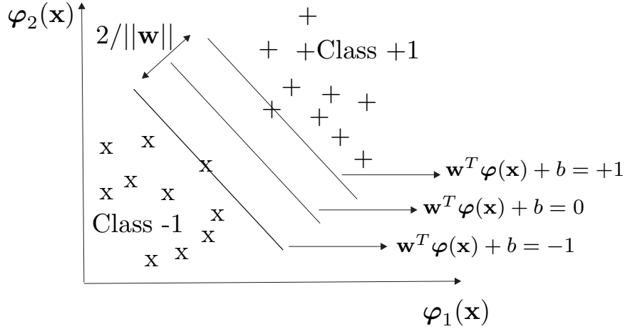
Figure 7: Illustration of SVM optimization of the margin in the feature space.
